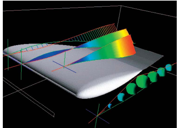
Figure 4: Comparing streamlines of two datasets simulated using different turbulence models. The streamlines are compared using line glyphs, strip envelopes, and sphere glyphs to highlight the differences between them. Image Courtesy of Alex Pang [VP04]
