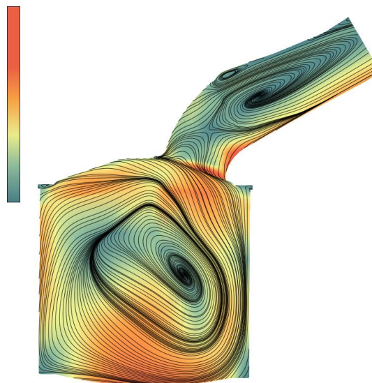
Figure 3: Visualization of flow through the gas engine simulation. By setting d_{rest} to 0.05 \times d_{sep} , streamlines overlay highlighting loops within the flow field. [SLCZ09]
