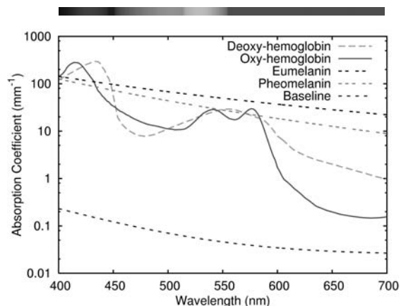
Figure 1: Spectral absorption coefficients of hemoglobin, melanins, and baseline skin absorption.
