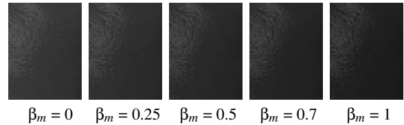
Figure 5: Change in skin color of a skin patch as the melanin blend \beta_m increases from 0 to 1. Lower values of \beta_m (more pheomelanin) give the skin a more yellowish appearance, while higher values (more eumelanin) give pure shades of tan and brown. The hemoglobin fraction C_h is constant at 0.1%, the total melanin volume fraction C_m is 50%, and the oiliness \rho_s is 0.5.
