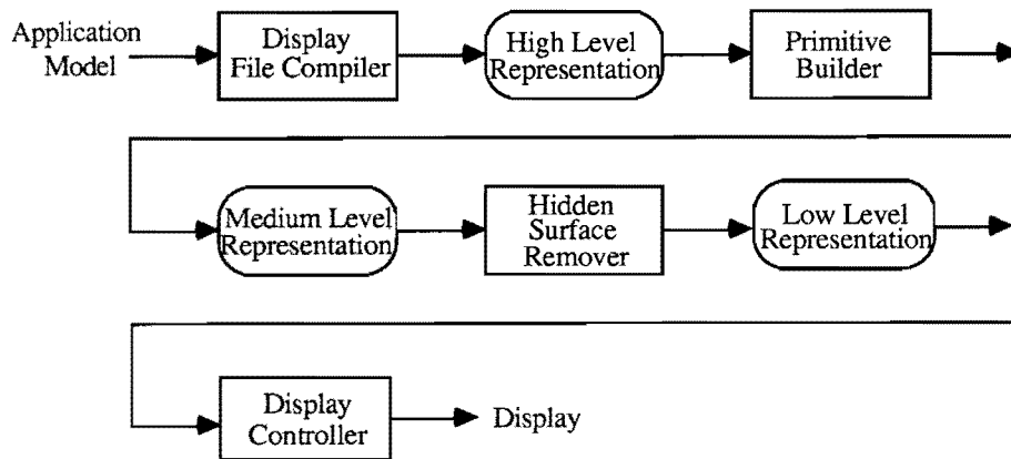
Figure 2: The proposed modified architecture.
