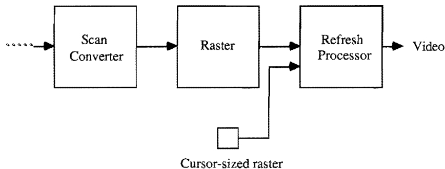
Figure 3: (Adapted from van Harmelen) A small raster for cursor feedback.
