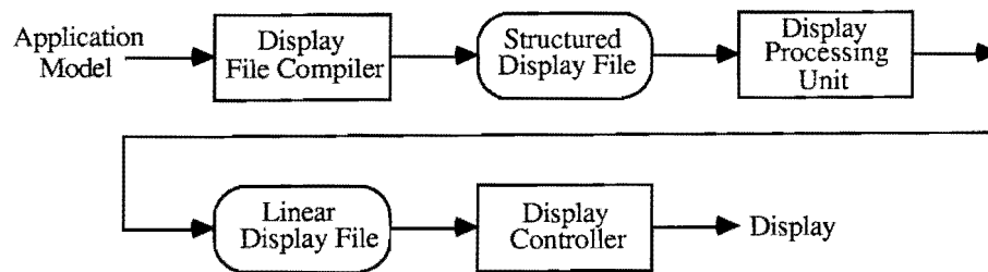
Figure 1: Carlbotm's classical architecture.
