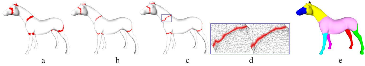
Figure 3: Post processing pipeline; interest regions (a), thinning (b), contour completion (c), snake movement (d), final segmentation (e).
