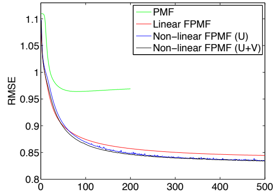
Figure 2: RMSE of validation set during training epochs
