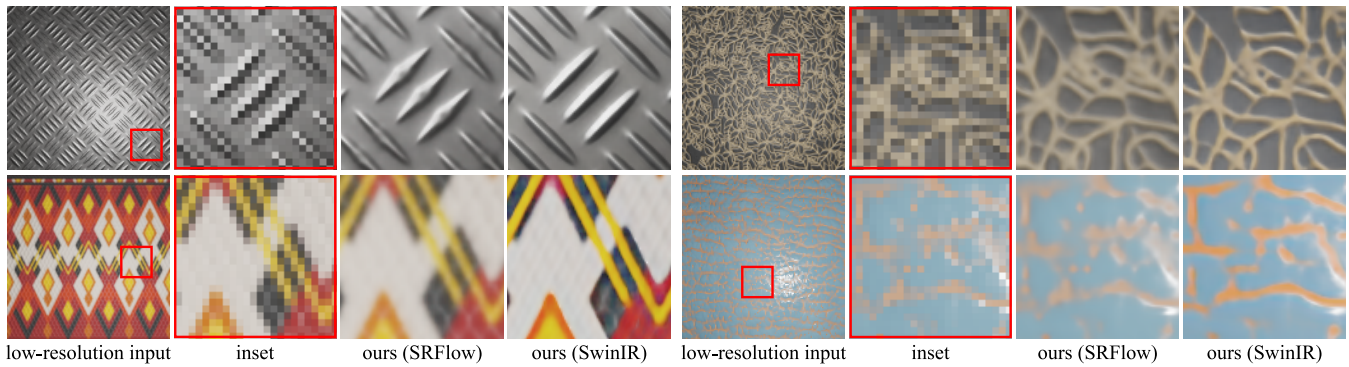
Figure 6: Comparisons between SRFlow [LDVGT20] and SwinIR [LCS*21] for upsampling SVBRDFs. Since each upsampler comes with its loss and training dataset, the upsampled renderings inherit from the upsamplers’ features. SRFlow tends to remain closer in appearance than SwinIR. The latter deviates from the original maps, producing sharper renderings and slight color shifts (best seen in the bottom row).
