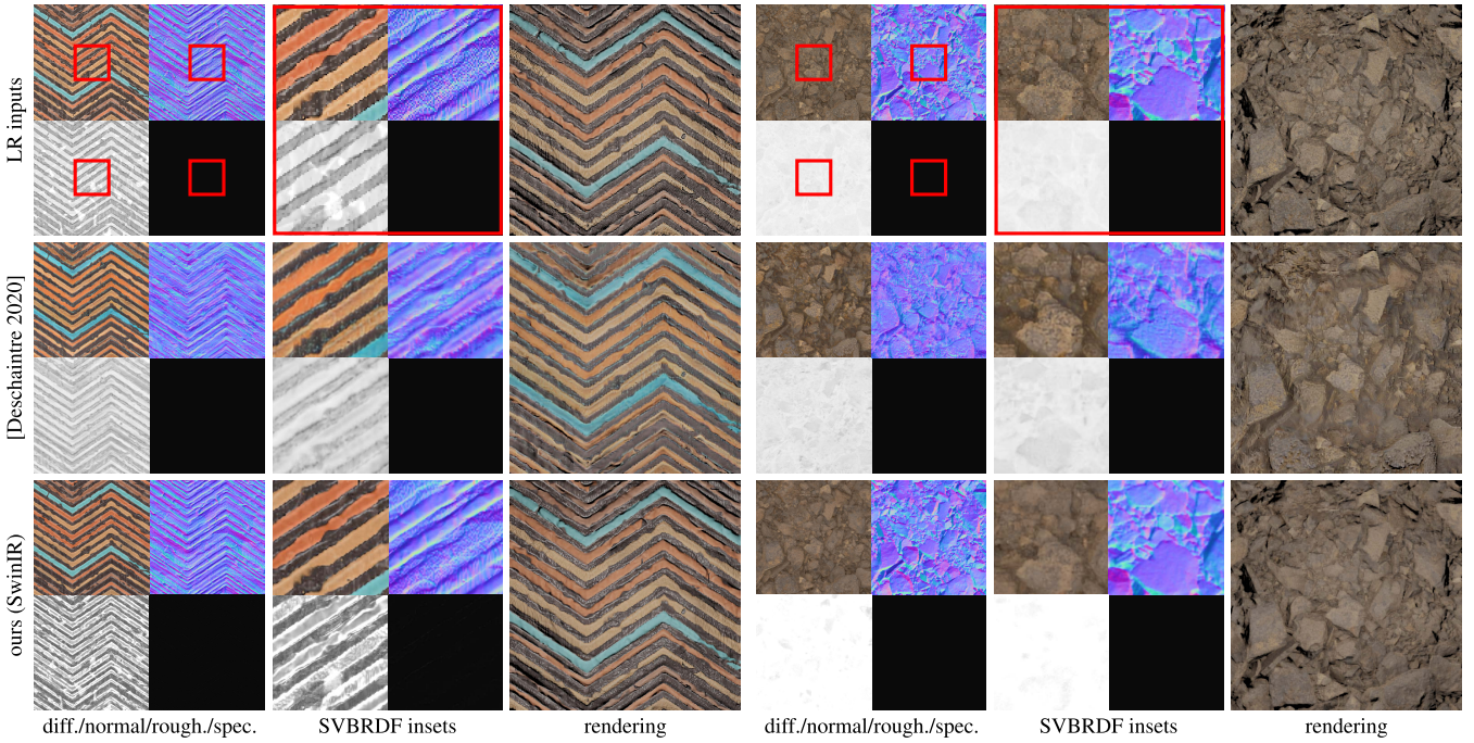
Figure 11: Comparisons with the approach of [DDB20]. The 1st row shows the LR finetuning guides and corresponding renderings. The estimated maps and renderings are shown in the 2nd row. As expected, the method is unable to provide consistent normals and bakes shading into the SVBRDF because of the lack of information coming from the single input. Our method (3rd row) better preserves the visual aspect of the material when rendered.
