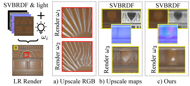
Figure 2: (Left) Given a Low-Resolution (LR) SVBRDF and a light direction \omega_i as input: a) Upscaling LR renders using SwinIR \times 4 [LCS*21] leads to inconsistencies (renders under \omega_1, \omega_2 ). b) Upscaling directly LR SVBRDFs using existing RGB-upsamplers is not appropriate, as these are designed to upscale radiances (or photographs). Notice how the structures do not overlap (SVBRDF and renders \omega_3 ). c) Given an RGB-upsampler S , we optimize for the upscaling of the input material, in order to retain S 's resolution enhancement capabilities in the shading.
