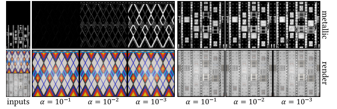
Figure 5: Comparisons between our inputs and the metalness and render outputs for varying \alpha . Our approach prevents value shifts while preserving the aspect of the rendered results.
