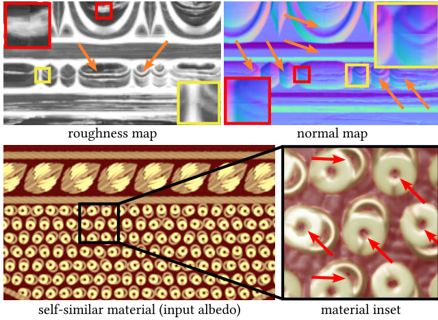
Figure 4: Limitations of a per-pixel approach. Top: discontinuities between adjacent tiles (orange) in the optimized roughness and normal maps . Bottom: rendering (right) showcasing inconsistent optimizations (red arrows) in a self-similar material (left) .
