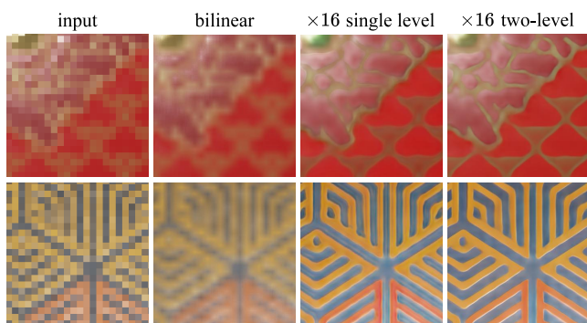
Figure 9: We achieve \times 16 super-resolution using SwinIR \times 4 by applying our neural filter twice to the input. The single level strategy provides usable SVBRDFs but the optimization of the second stage in the two-level strategy brings sharper structures and fewer artifacts.
