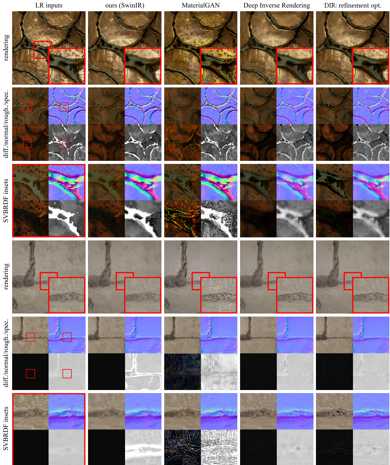
Figure 13: Comparison with MaterialGAN [GSH*20] and Deep Inverse Rendering [GLD*19]. MaterialGAN (3rd column) exhibits noise, renderings artifacts, and the concatenation of independently upsampled patches leads to visible seams. Deep Inverse Rendering’s inversion in the latent space (4th column) leads to biased and blurry SVBRDF, which the refinement step (last column) improves, at the cost of noise. The refinement cannot improve the biased output of the inversion step (see 3rd row), but create sharper results, as shown in both refined outputs materials.
