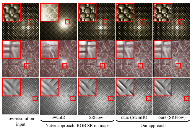
Figure 10: Direct super-resolution of SVBRDF maps using ML-based RGB upsamplers ( 2^{\text{nd}} and 3^{\text{rd}} columns) is not viable, as material maps differ in nature, geometric constraints and statistics from RGB photographs. All maps contribute also in a very different manner to and have a different impact on the final shading.
