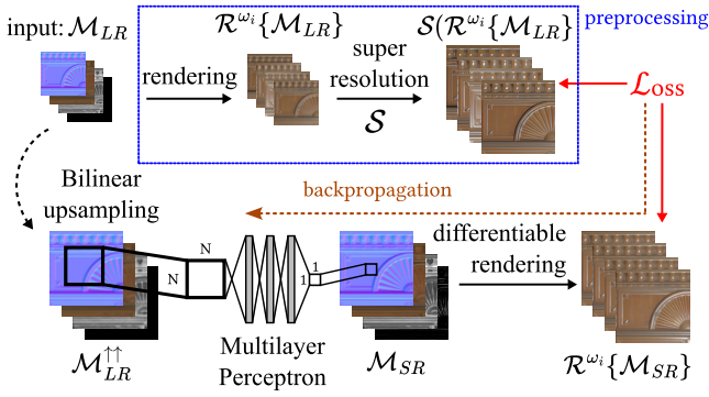
Figure 3: Overview of our method for radiance-based SVBRDF super-resolution. The main metaparameters of our approach are a shading model \mathcal{R} , a super-resolution algorithm \mathcal{S} , and a tile size N .
