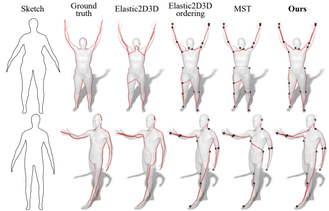
Figure 14: Examples of how our curve reconstruction method is applied to refine a contour. Given a contour obtained with ELASTIC2D3D [LRS* 16], we sample it sparsely and reconnect the samples using the ordering of the contour, MST, and our algorithm.
