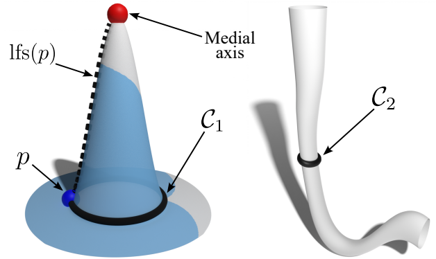
Figure 5: Two examples of curves on surfaces (solid black) where the local feature size exhibits undesired behaviors. Left: an r -ball (shaded in light blue) around p that contains the entire curve \mathcal{C}_1 , but no point of the medial axis. Right: a curve \mathcal{C}_2 on the surface with an empty medial axis (i.e., the local feature size is undefined).
