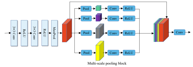
Figure 5: The structure of multi-scale convolution block in MEncoder.
