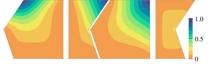
Figure 2: Examples of BMLC for a convex and a concave polygon.
