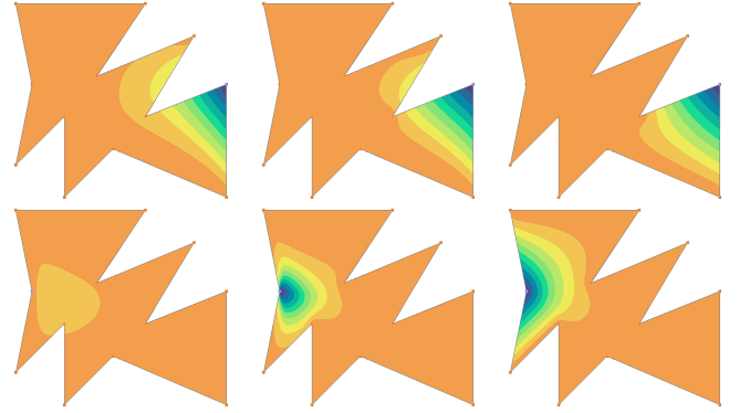
Figure 4: Examples of BMLC (left), MLC with projection (middle), and MLC with projection and smoothing (right).
