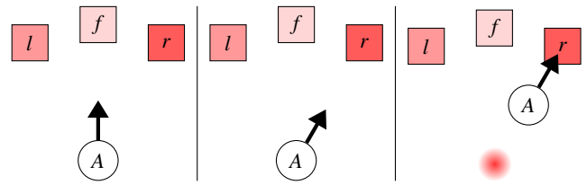
Figure 3: The behavior of a slime agent A. The agent samples from three sensors in front of it (left l, right r, and forward f) and determines the next direction by choosing the one with highest pheromone concentration (darker red). When leaving a location, the agent releases pheromone.
