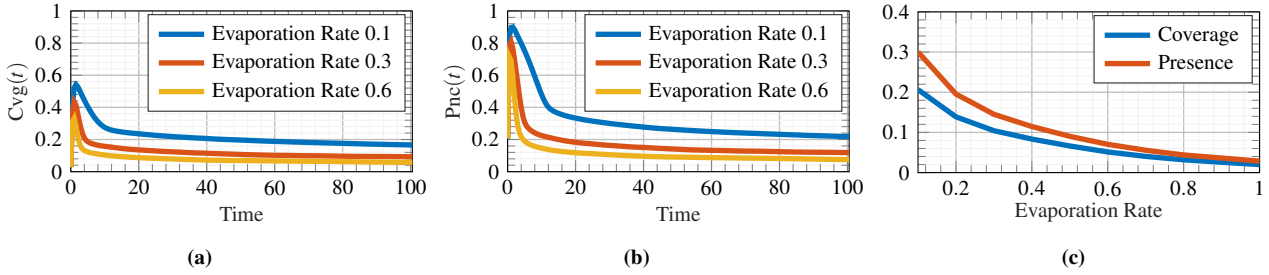
Figure 8: Evolution of the pheromone coverage (a) and presence (b) during a simulation of 100 seconds. After the initial peak, the agents stabilize on the pattern family and slowly vary the resulting pattern. Different decay rates shift the curve, without changing the evolution. The pheromone coverage and presence after 70 seconds of simulation vary as the decay rate changes (c). The slower the evaporation, the higher the coverage and presence. We performed these experiments on the shape on the left of Figure 1.
