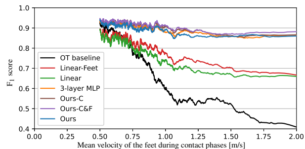
Figure 8: F_1 score against amount of footskate. Test motions with matching foot contact patterns have been blended to purposely introduce footskate while preserving contact labels. Foot contact detection is then evaluated on such motions suffering from footskate, and compared to the ground truth contact labels. The amount of footskate introduced through blending is measure using the mean velocity of the feet during contact phases. Non-linear learned detection models keep reasonably high accuracy while accuracy of linear models significantly decrease and accuracy of OT baseline quickly collapse.
