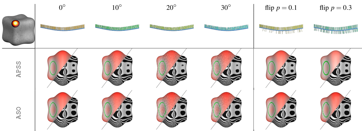
Figure 6: Stability of APSS and ASO on perturbed normal vector field input: using similar rendering as for Figure 5, we compared estimated quantities when normal vectors are perturbed using a random angular Gaussian noise of degrees in \{0, 10, 20, 30\} around the exact normal vectors, or when the normal vectors are flipped with probability 0.1 and 0.3.
