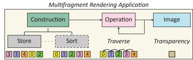
Figure 2: Diagram of building an application using the MFR pipeline (top). Order-independent transparency requires the sorting of an arbitrary sequence of out-of-order fragments before alpha compositing them in a linear traversal fashion (bottom).
