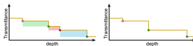
Figure 11: The visibility function models how light is absorbed as it travels through space (left). To compress this, the fragment that generates the smallest area variation is removed [SML11] (right).
