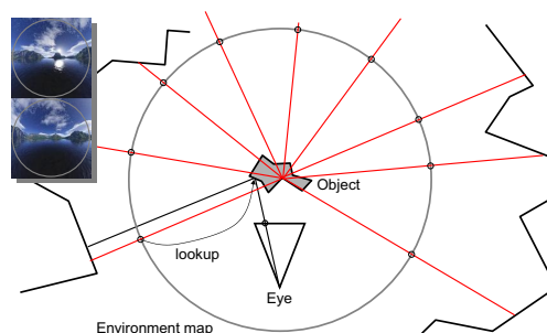
Figure 12: Radiance incident at a single point is stored in an environment map. Here, we have used the parabolic parameterization 28 to store the incident radiance.
