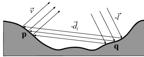
Figure 10: Light is reflected at point q towards point p and is then reflected towards the viewer.
