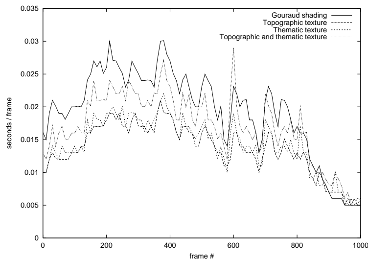
Fig. 7. Timings for different visualization techniques
