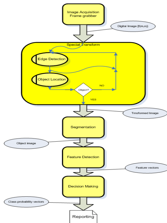
Figure 2: Recognition processes.
