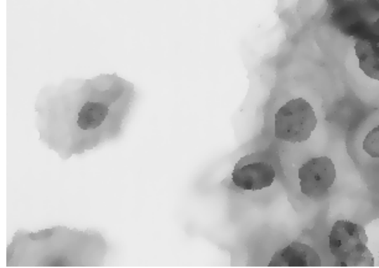
Figure 9: Filtered image.
