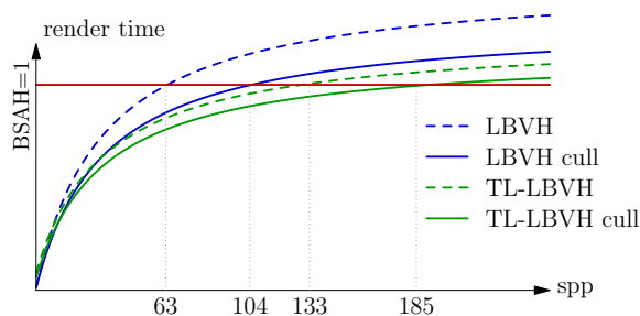
Figure 7: Render times for increasing number of shadow samples per pixel normalized to ray tracing using BSAH. With large enough sample count the impact of hierarchy construction diminishes. However, while staying in the realm of interactive rendering sub-optimal hierarchies perform better regarding time-to-image.
