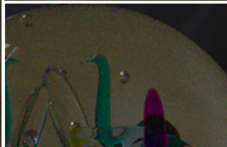
PSSMLT 0.5
