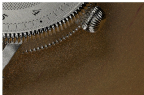
Ground truth
