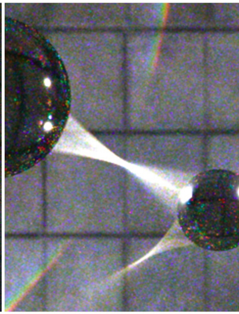
PSSMLT 0.75
