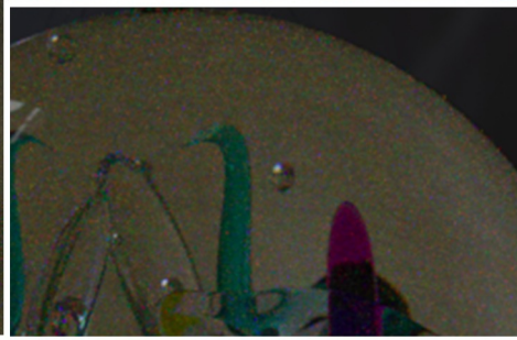
PSSMLT 0.75
