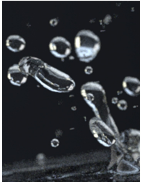
PSSMLT 0.5
