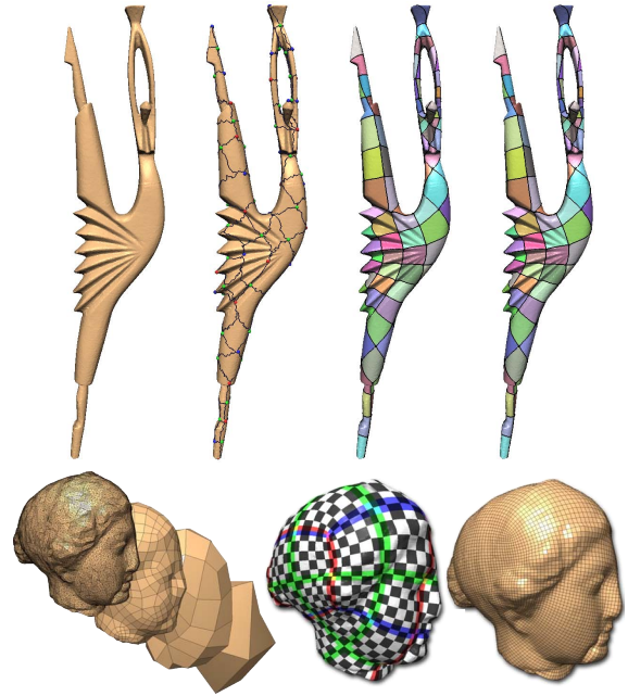
Figure 5: Top: different phases composing [DBG*06]; given a triangle mesh, an initial Morse-Smale complex is extracted, then boundaries are improved through a sequence of relaxation steps, this finally allows to gather a high quality quadrangulated model. Bottom: The step composing [DISC09b]; a base domain is obtained through a sequence of simplification operations, original vertices were mapped to the base domain, then sampling the base domain is possible to gather a semiangular quad mesh.
