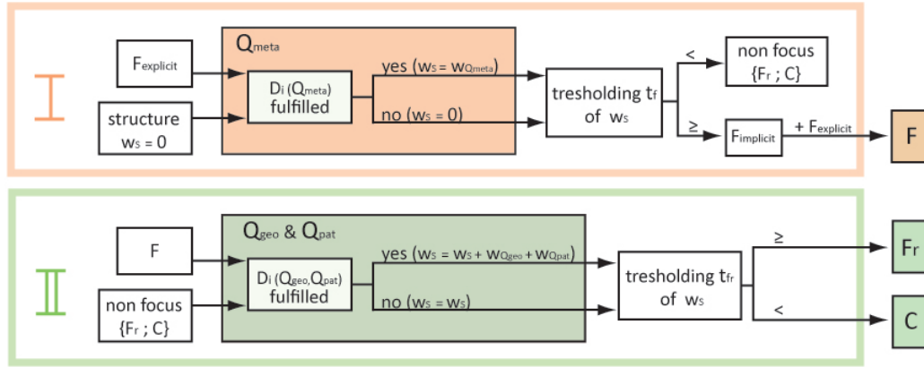
Figure 3: The two step categorization pipeline. Step I identifies the focus structures F by using the meta information ( Q_{meta} ) of the current question. With conditions D_i(Q_{meta}) and weights w_{Q_{meta}} the structure's weight w_s and, thus, importance is determined. The thresholding of w_s realizes the first categorization in focus F and non focus. All structures \in \{F_r; C\} will be analyzed in step II with Q_{geo} and Q_{pat} . The conditions D_i(Q_{geo}, Q_{pat}) are evaluated and the individual structure's importance is adapted. A thresholding is performed similar to step I to classify focus relevant F_r and context C structures.
