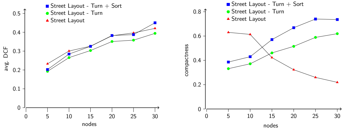
Figure 6: Comparison of stability (left) and compactness (right) between Street Layout, Street Layout with turning side streets and additional sorting based on flat hierarchies with increasing width.
