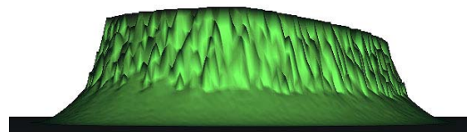
Figure 1: Photograph of a table mountain (left) and the model obtained by erosion simulation
