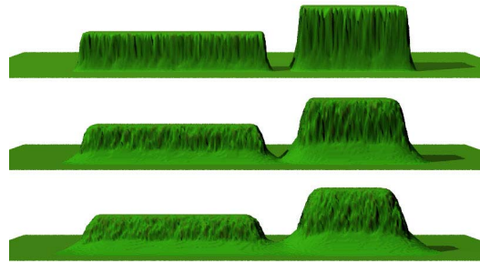
Figure 9: Erosion of a regular shape leads to a visually realistic result
