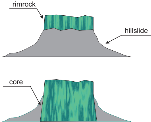
Figure 3: Table mountain shape (top) and its inner structure (bottom)
