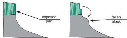
Figure 4: The hard→soft erosion process
