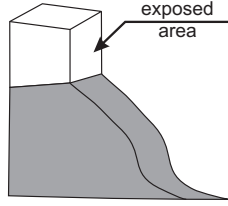
Figure 5: The exposed area of a rimrock
