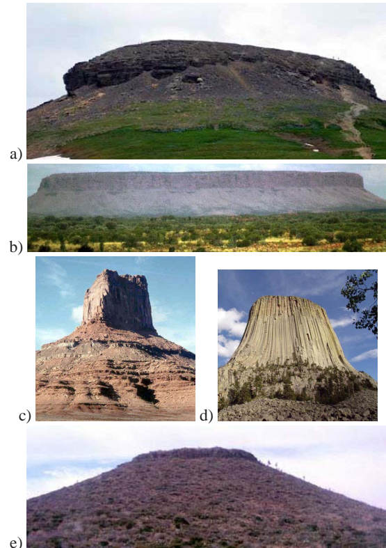
Figure 2: Table mountains. a) Small hill b) Table Mountain (Cape Town) c) White Rim (SF), d) Devils Tower (WYO) e) Zacatecas desert table mountain (Mexico)
