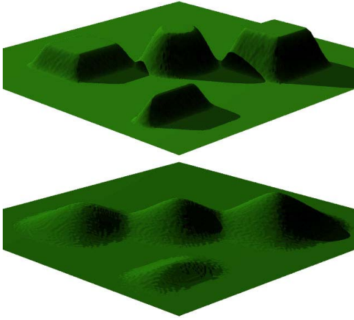
Figure 8: Erosion of the soft material
