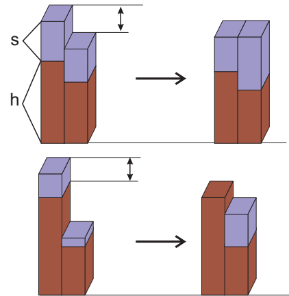
Figure 7: Two possible cases of the soft material transportation
