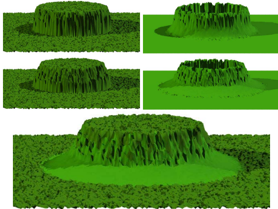
Figure 6: Thinning of the core (left) of a mountain caused by erosion. The soft layer is displayed in the right column and both layers in the last image
