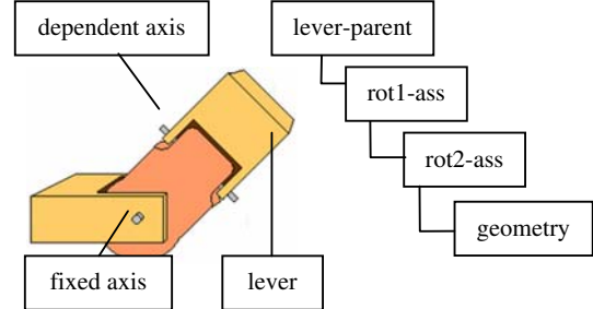
Figure 13: Schematic structure of two-dof joints and their representation in the scene graph
