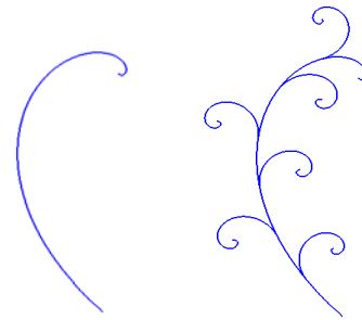
Figure 2: Left: a single curve; right: six new curves growing from the left initial curve.
