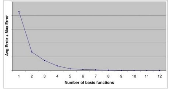
Figure 3: The error the choice of basis functions used to fit the BRDFs in the database.
