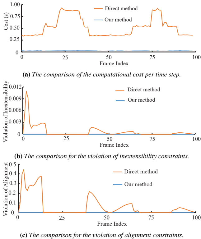
Figure 10: Comparison between our method and the direct KKT method in Cartesian coordinates. We simulate helix under gravity as shown in Fig. 6. Our method not only spends less time than constructing KKT system and solving it in Cartesian coordinates (a) but also satisfies all the nonlinear intrinsic constraints (see (b) and (c)).
