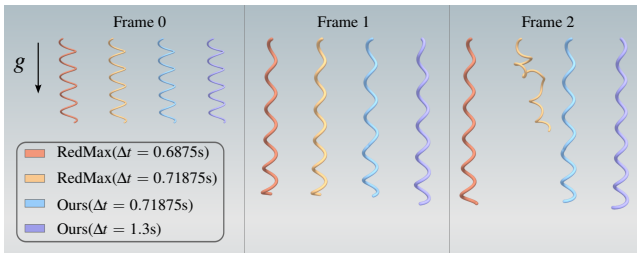
(b) The helix under gravity by our method and extended RedMax.
