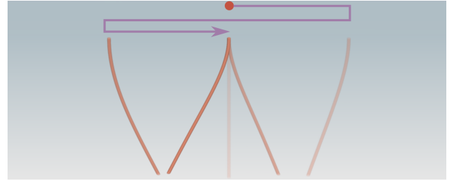
Figure 11: Dragging the root of a rod. We simulate the rod using 200 segments, with 1m as reference length, 1 \text{ kg/m}^3 as density, 0.03 m as radius, 1 MPa as Young's modulus, 1 MPa as shear modulus, and \Delta t = 250 ms. We move two vertices on the top of the rod in a sine wave and the displacement of the top two vertices can be analytically expressed as \phi \sin(2\pi ft) . We set f = 1 and \phi = 0.5 m, which is the half of the reference length of the rod.
